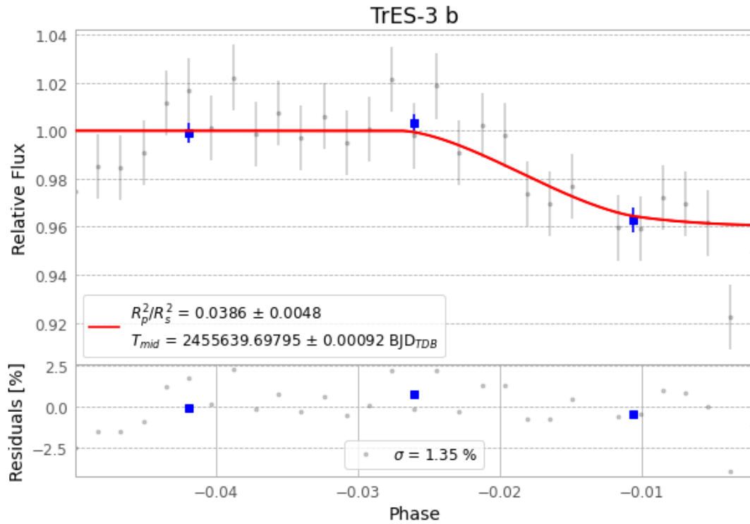
Figure 1 — FinalLightCurve_TrES-3 b_2011-03-20.png (SHA-256 c31f2cb927691b36...)
