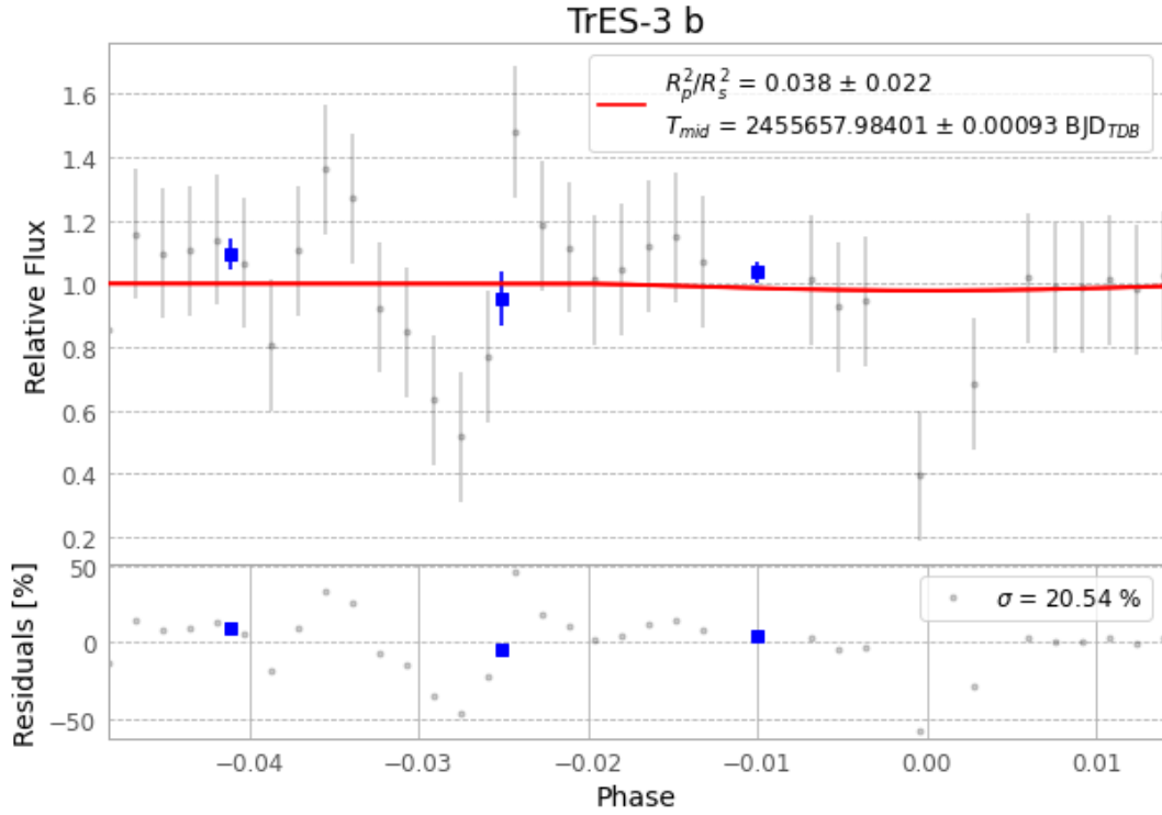
Figure 1 — FinalLightCurve_TrES-3 b_2011-04-06.png (SHA-256 e58321b892530dc7...)
