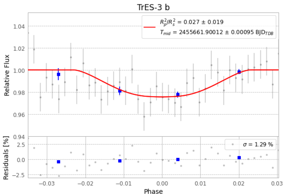
Figure 1 — FinalLightCurve_TrES-3 b_2011-04-10.png (SHA-256 a6ac63e1c7d5fc70...)
