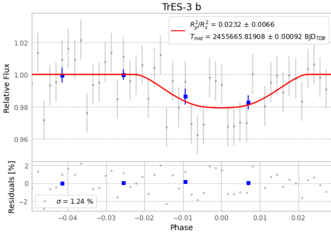
Figure 1 — FinalLightCurve_TrES-3 b_2011-04-13.png (SHA-256 3241adf0c10d1cd0...)
