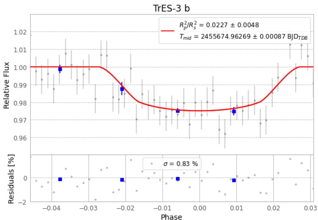
Figure 1 — FinalLightCurve_TrES-3 b_2011-04-23.png (SHA-256 4e8d94da02f711c7...)
