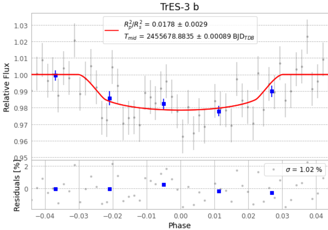
Figure 1 — FinalLightCurve_TrES-3 b_2011-04-27.png (SHA-256 eb3c280c53a53eba...)
