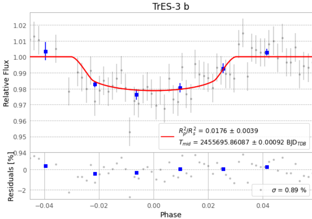
Figure 1 — FinalLightCurve_TrES-3 b_2011-05-14.png (SHA-256 2b209b4400420f5e...)
