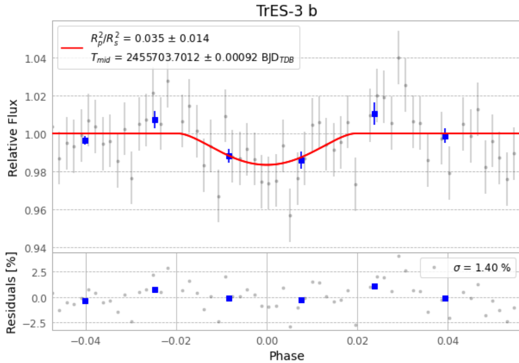
Figure 1 — FinalLightCurve_TrES-3 b_2011-05-21.png (SHA-256 09319693d55065cf...)
