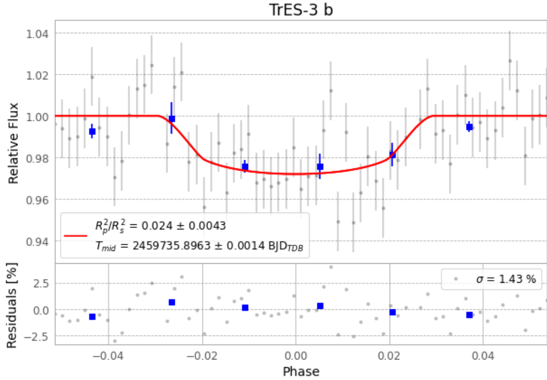
Figure 1 — FinalLightCurve_TrES-3 b_2022-06-05.png (SHA-256 30a6a0d9a18ad385...)
