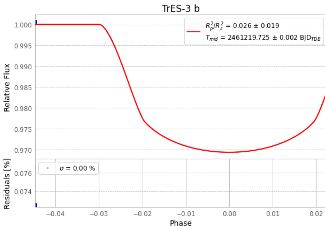
Figure 1 — FinalLightCurve_TrES-3 b_2026-06-27.png (SHA-256 f0cf70091816bb5f...)
