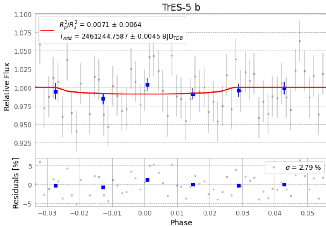
Figure 1 — FinalLightCurve_TrES-5 b_2026-07-22.png (SHA-256 b363482abb9f6df3...)
