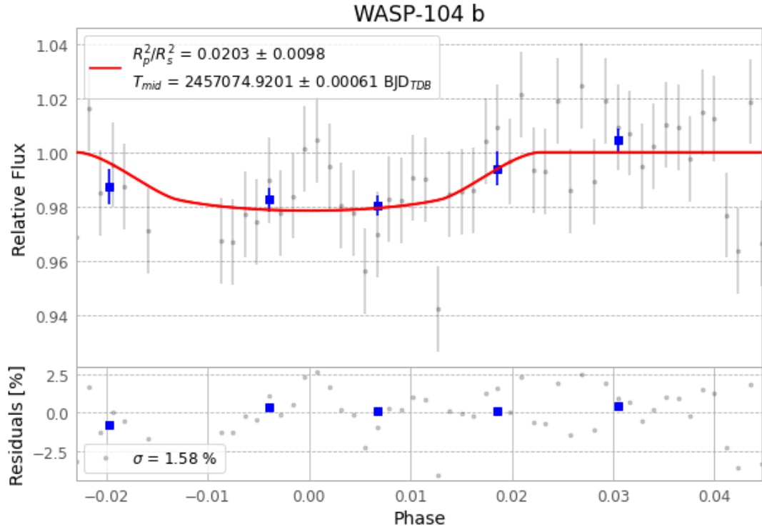
Figure 1 — FinalLightCurve_WASP-104 b_2015-02-21.png (SHA-256 98fdf2b9793364b1...)
