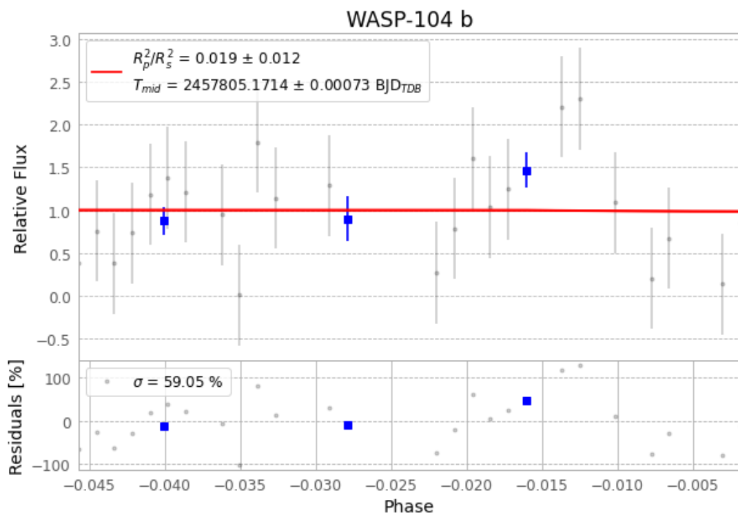
Figure 1 — FinalLightCurve_WASP-104 b_2017-02-22.png (SHA-256 9b2be5cd2239b8c7...)
