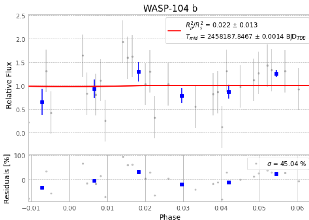
Figure 1 — FinalLightCurve_WASP-104 b_2018-03-10.png (SHA-256 38ab9d1569ffbd1b...)
