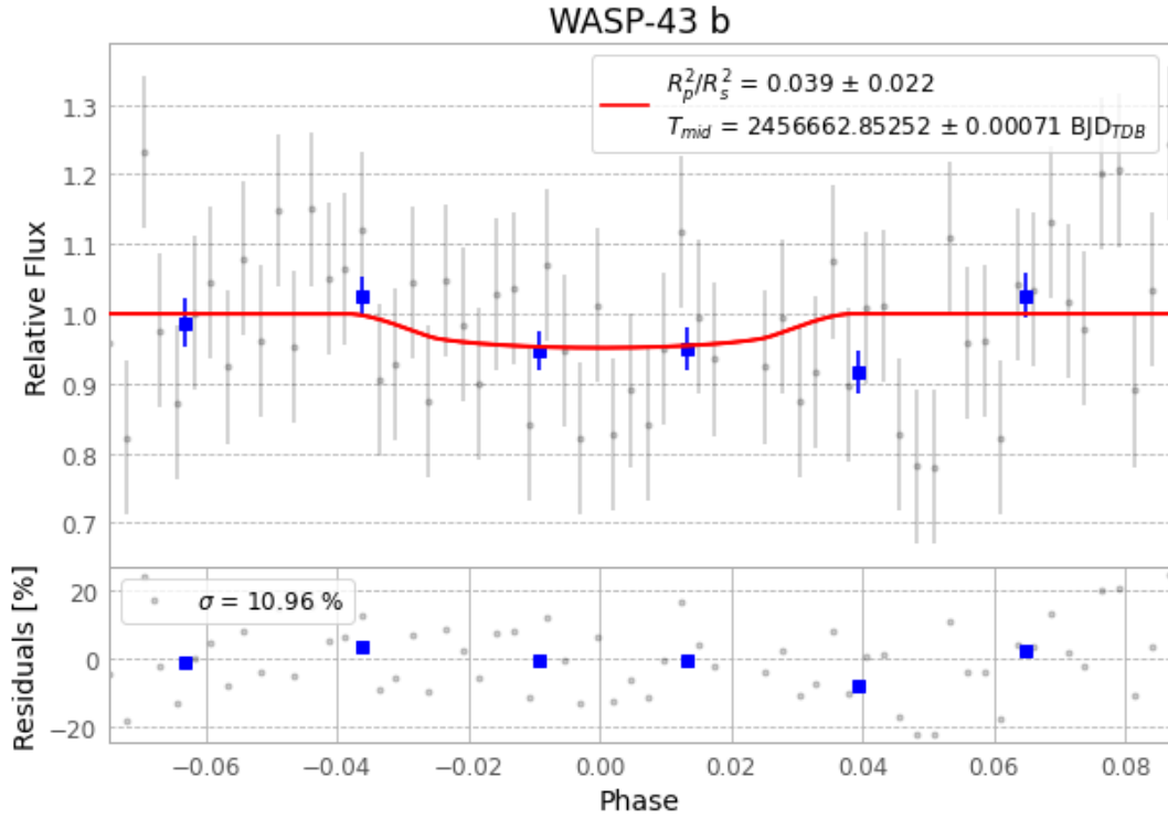
Figure 1 — FinalLightCurve_WASP-43 b_2014-01-04.png (SHA-256 9cf26ebfda48da70...)
