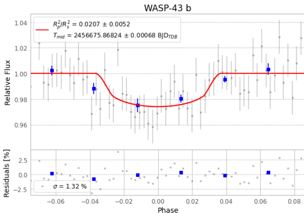
Figure 1 — FinalLightCurve_WASP-43 b_2014-01-18.png (SHA-256 1e0ca77f52cf7514...)
