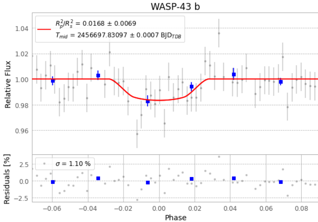
Figure 1 — FinalLightCurve_WASP-43 b_2014-02-08.png (SHA-256 ace6142a18034668...)
