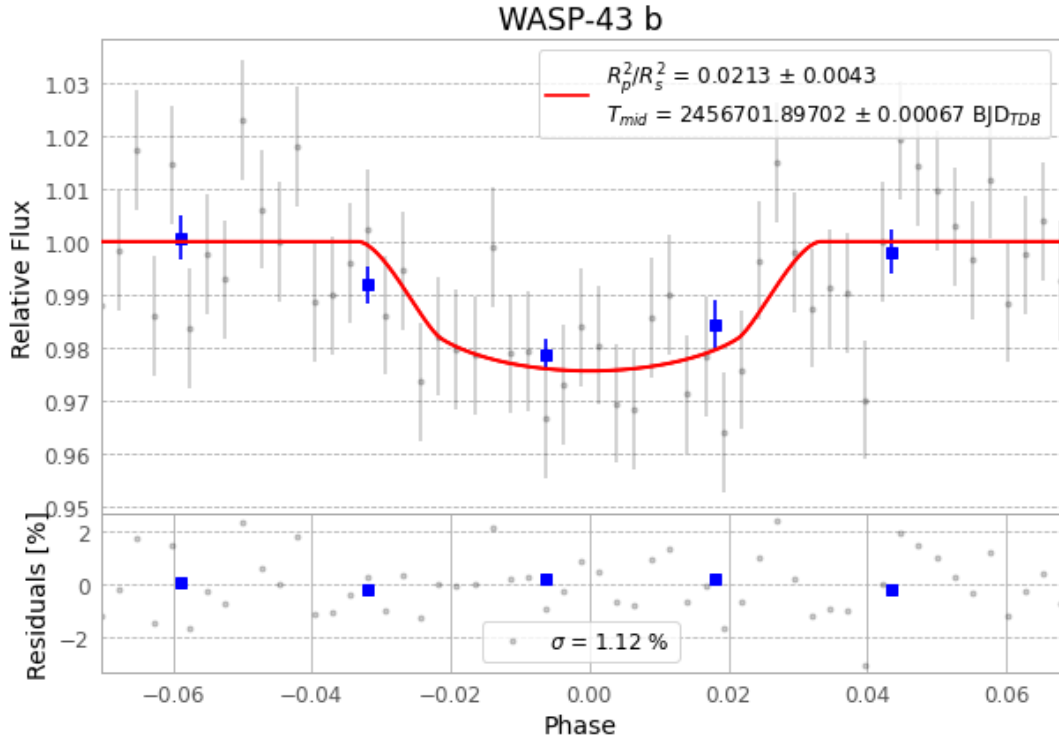
Figure 1 — FinalLightCurve_WASP-43 b_2014-02-13.png (SHA-256 ba3c357a9b1240a6...)
