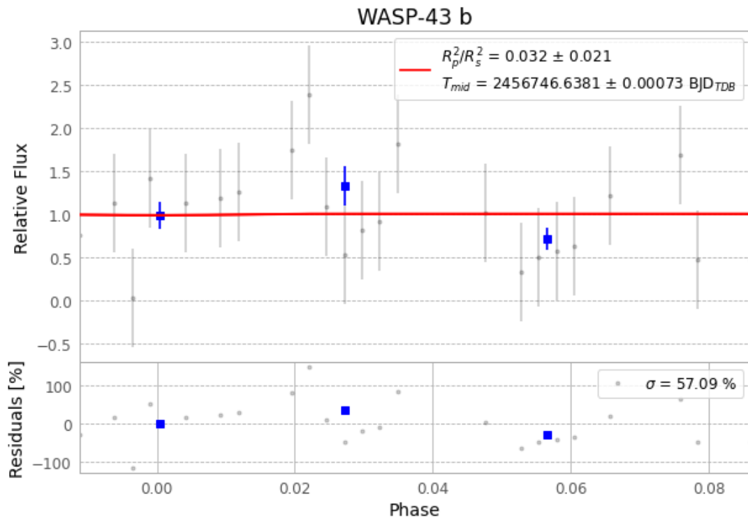
Figure 1 — FinalLightCurve_WASP-43 b_2014-03-29.png (SHA-256 69866013bd26dd66...)
