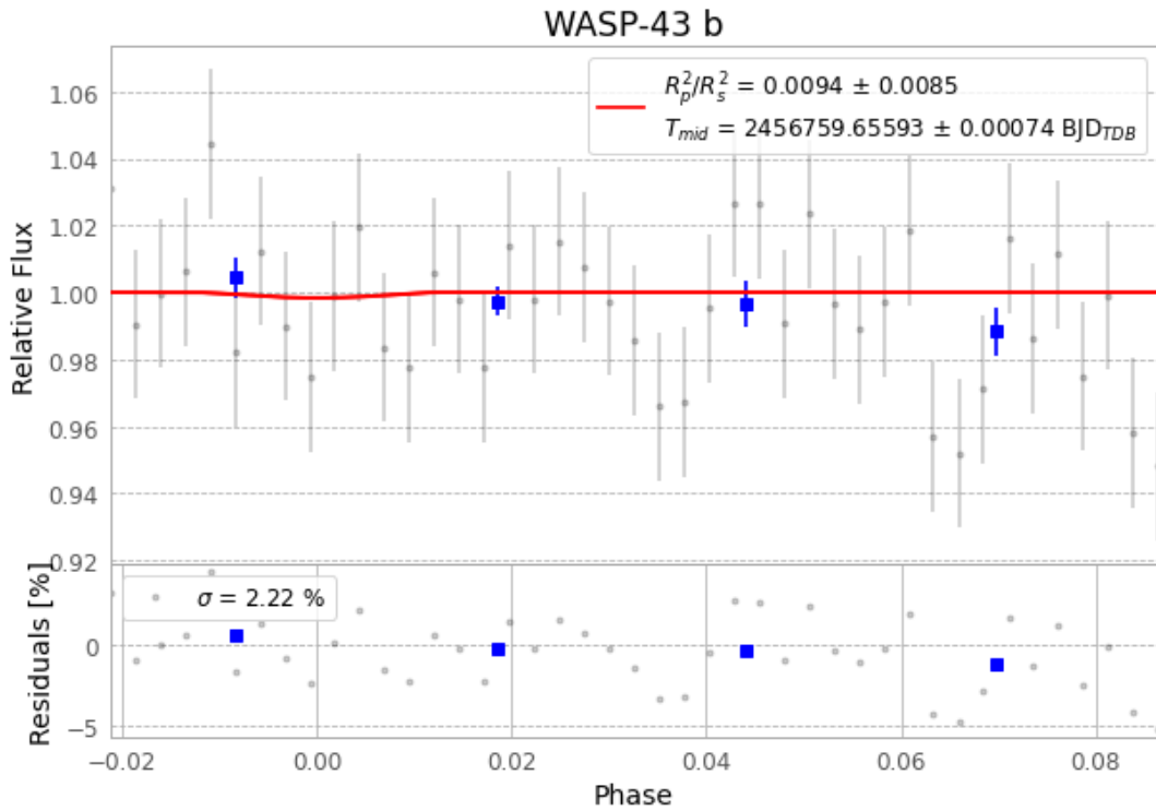
Figure 1 — FinalLightCurve_WASP-43 b_2014-04-11.png (SHA-256 d2f391e284a68213...)
