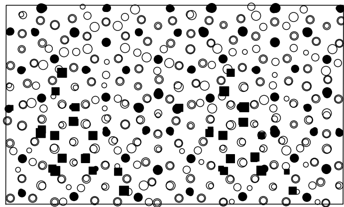
(b) W-phase, 530 atoms in the conventional cell
