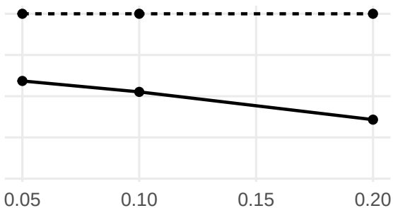
Exchangeable logistic-normal (refit); rho
