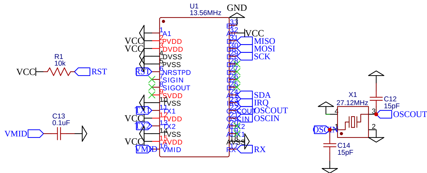
MFRC522
