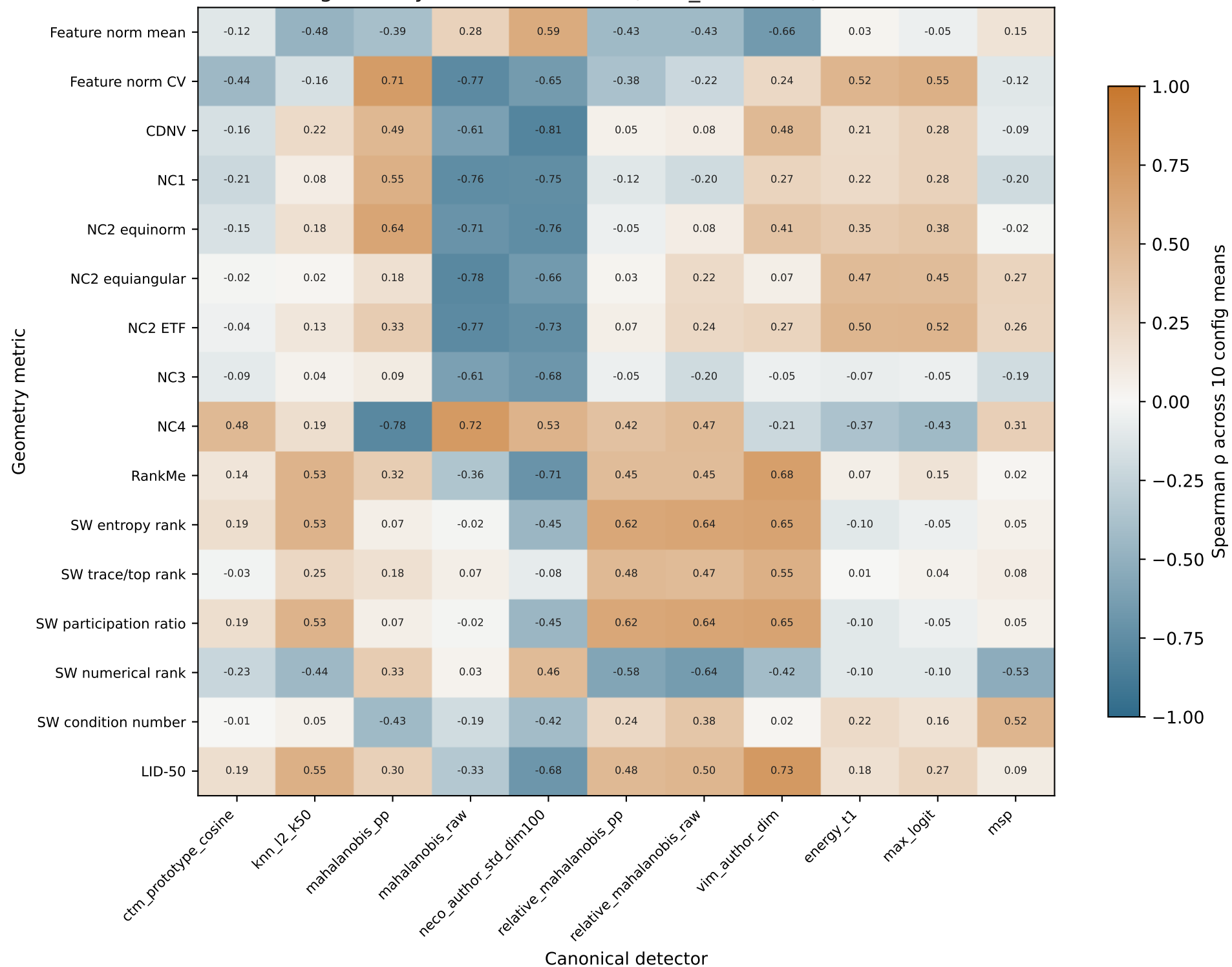
Places365 geometry-OOD association (best_val, auroc)
