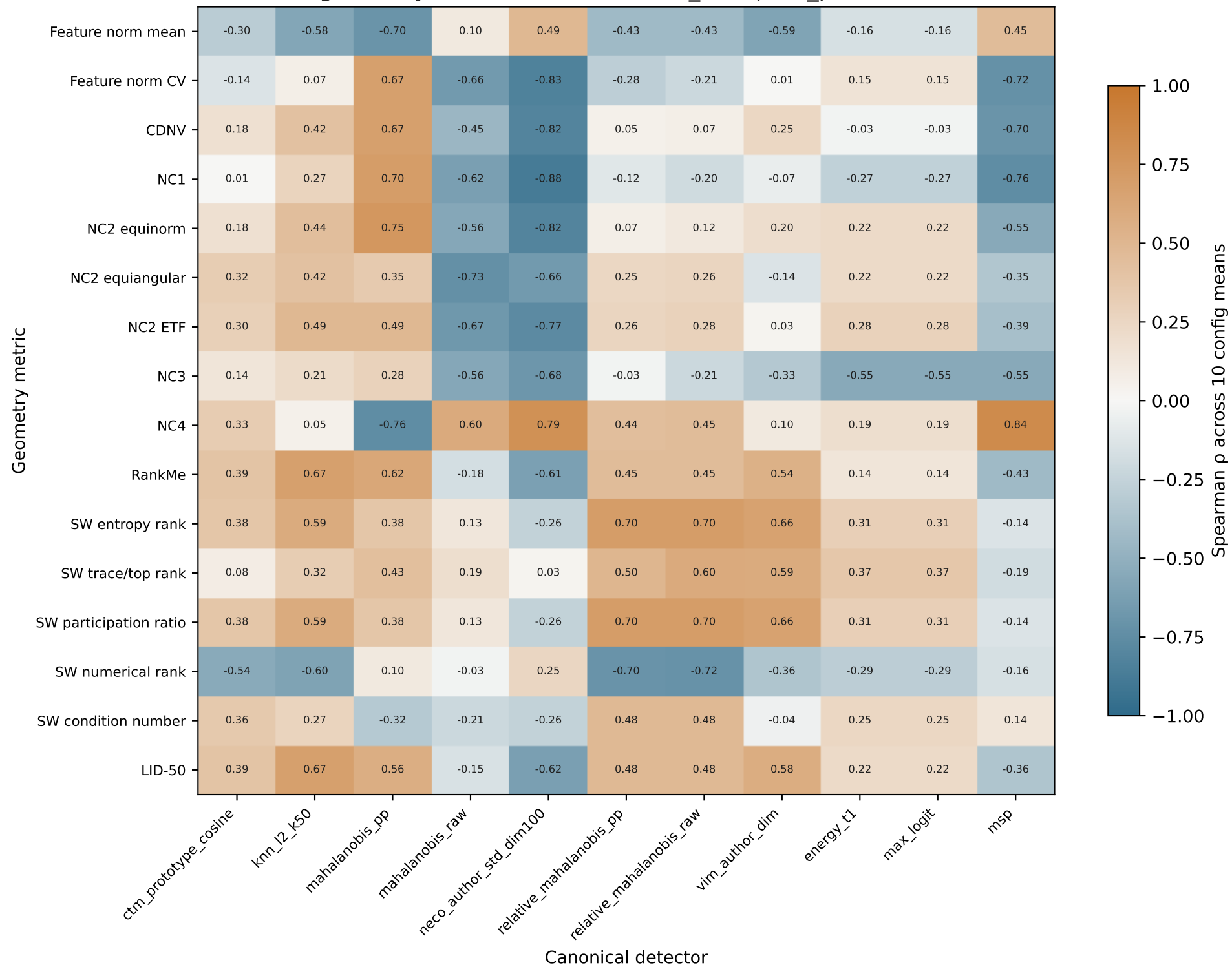
Places365 geometry-OOD association (best_val, fpr95_performance)
