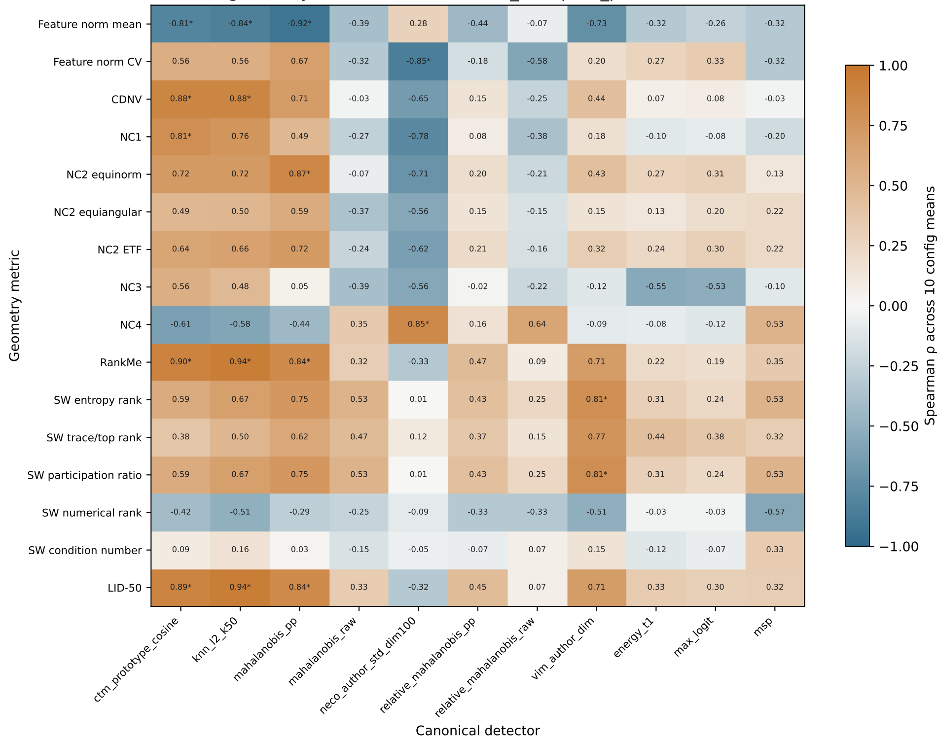
Textures geometry-OOD association (best_val, fpr95_performance)
