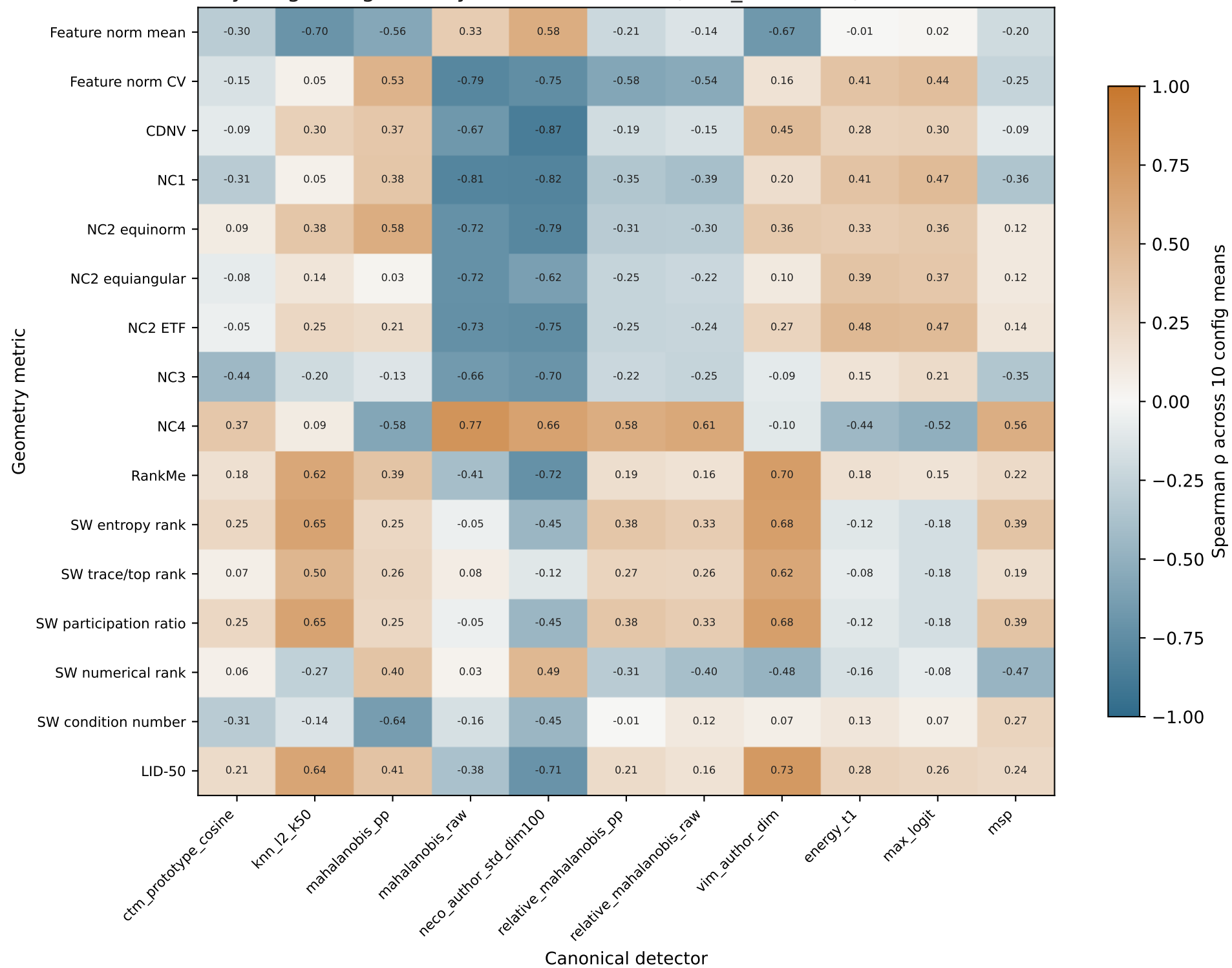
TinyImageNet geometry-OOD association (best_val, auroc)
