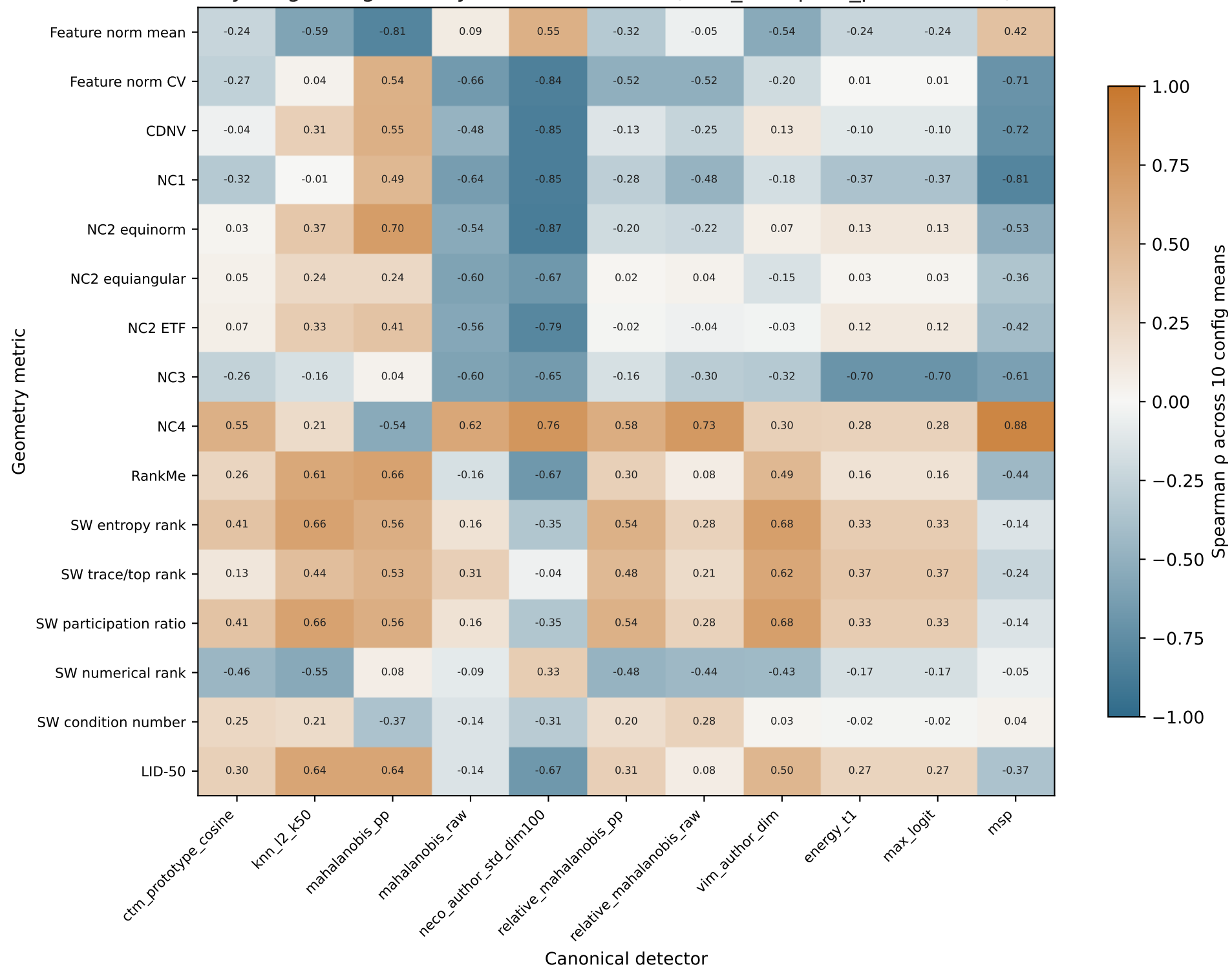
TinyImageNet geometry-OOD association (best_val, fpr95_performance)
