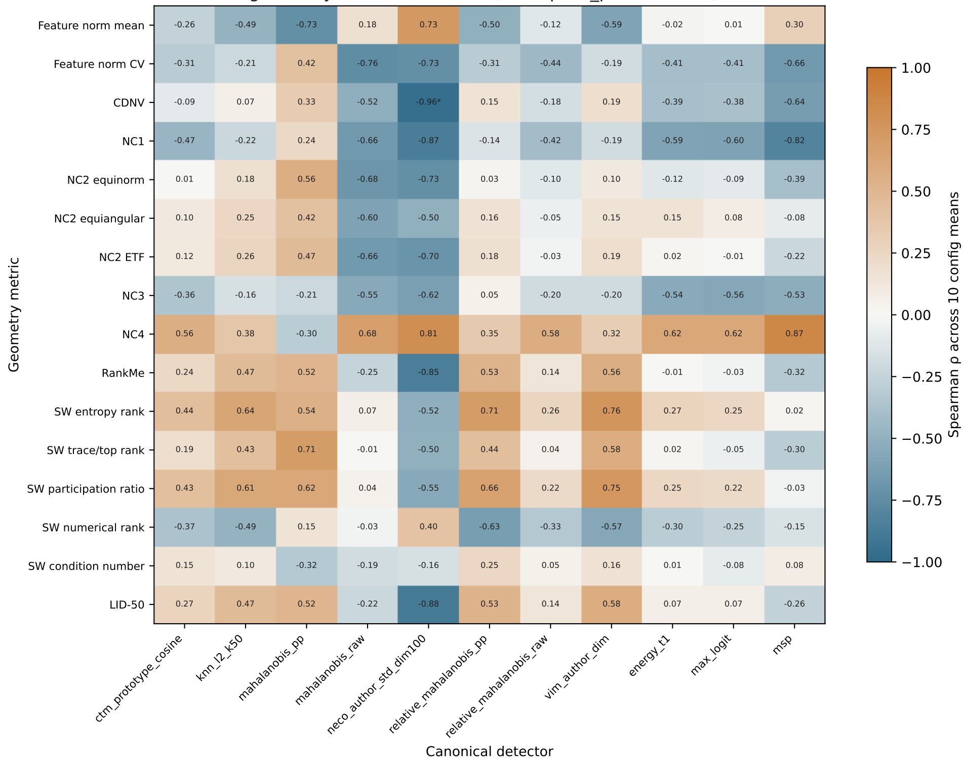
CIFAR-100 geometry-OOD association (last, fpr95_performance)
