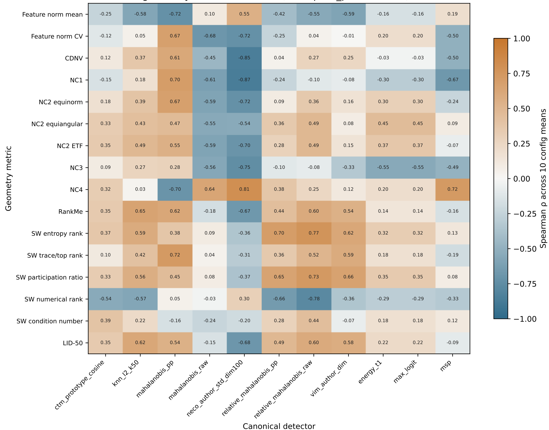
Places365 geometry-OOD association (last, fpr95_performance)
