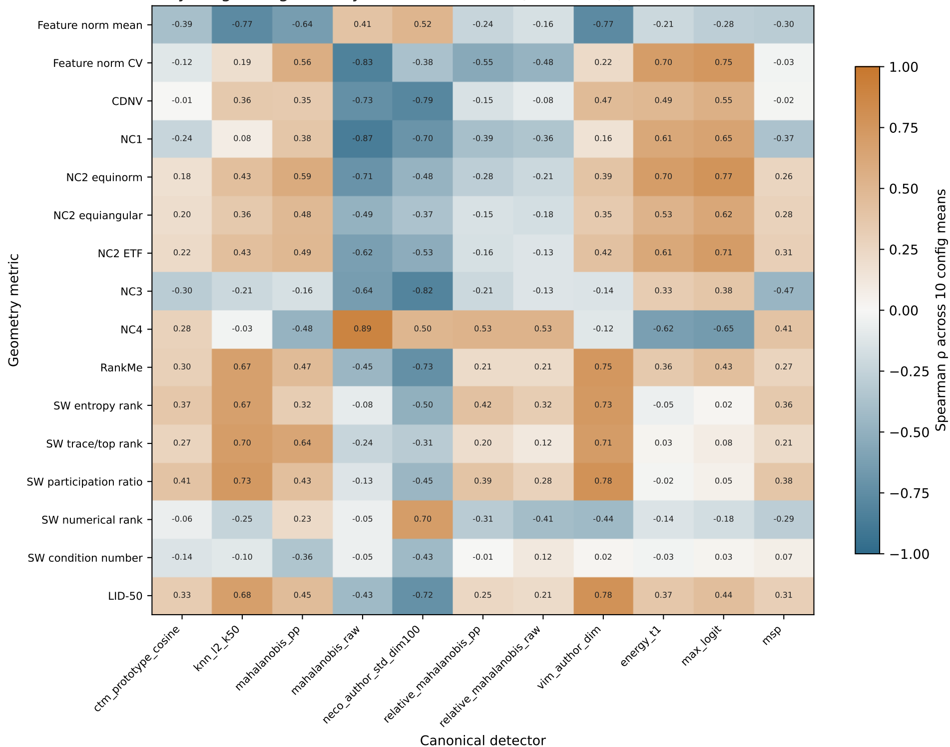
TinyImageNet geometry-OOD association (last, auroc)
