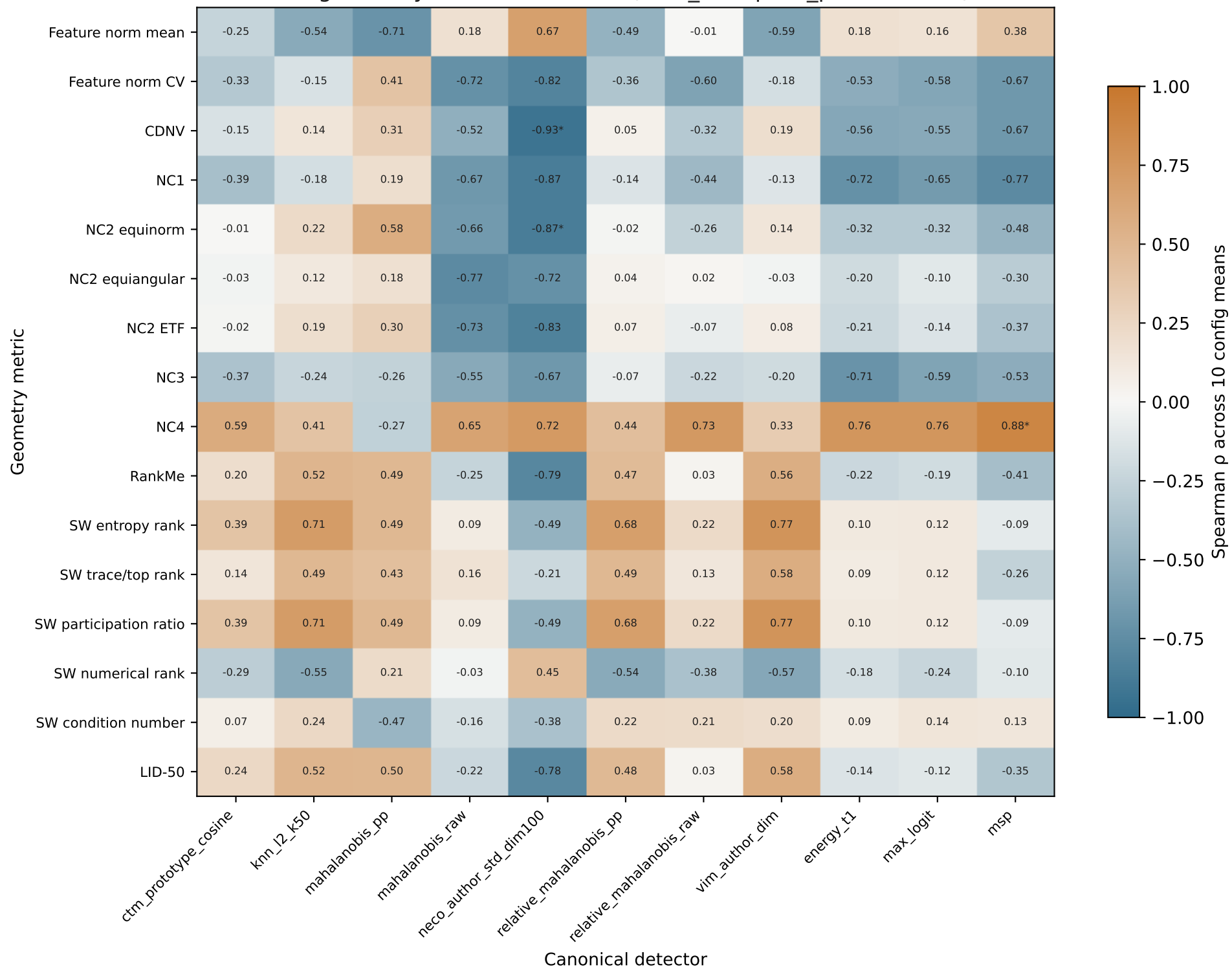
CIFAR-100 geometry-OOD association (best_val, fpr95_performance)
