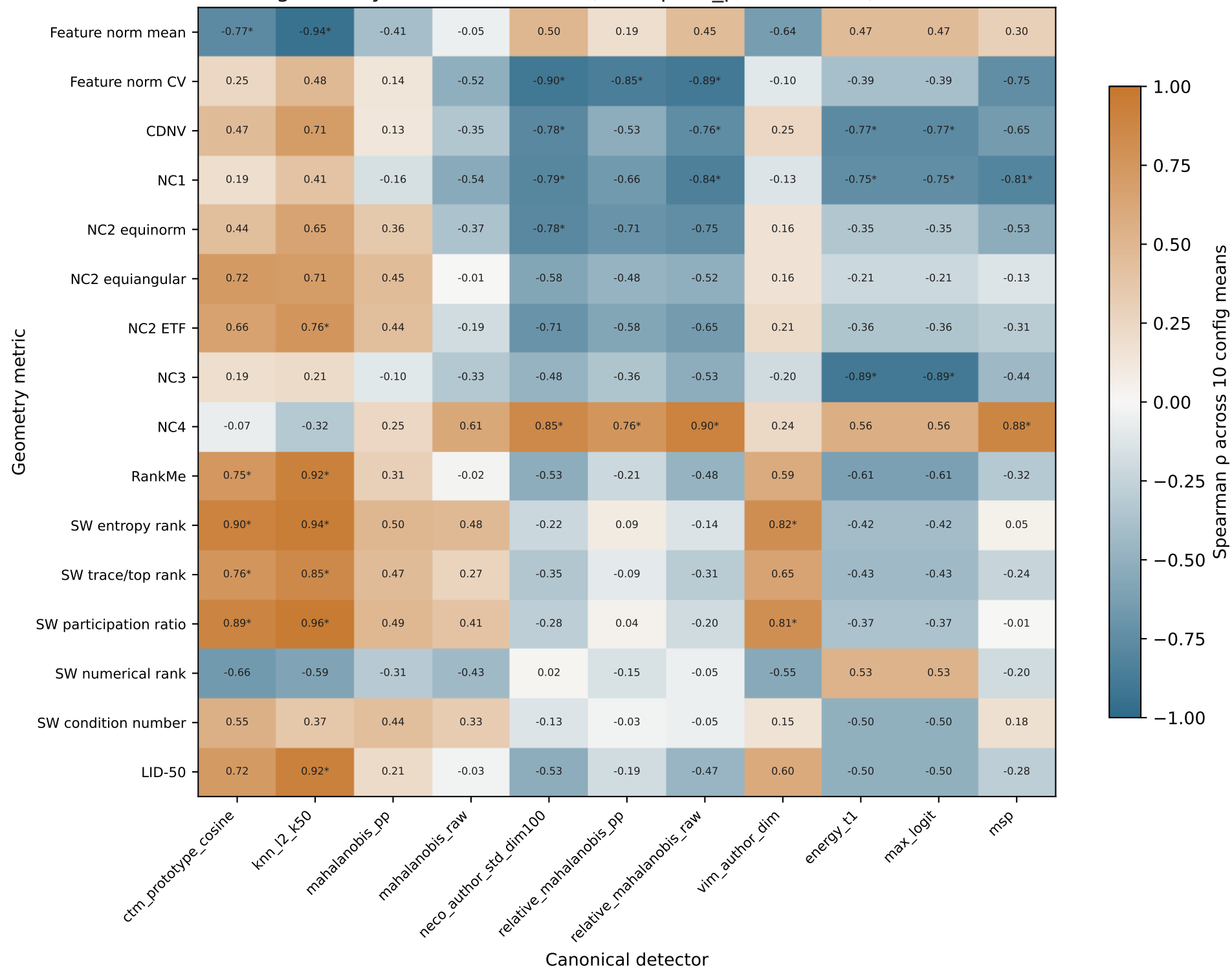
MNIST geometry-OOD association (last, fpr95_performance)
