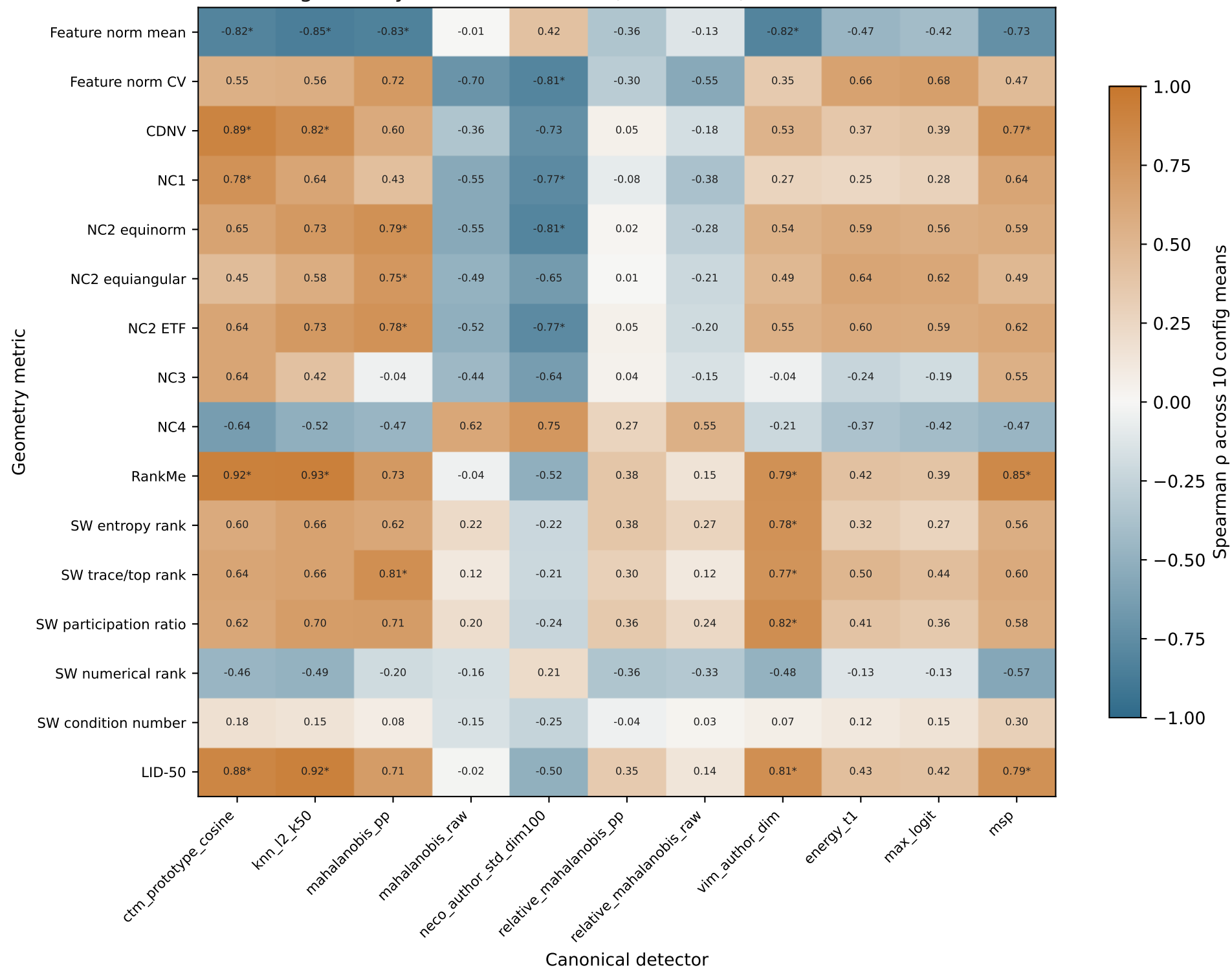
Textures geometry-OOD association (last, auroc)
