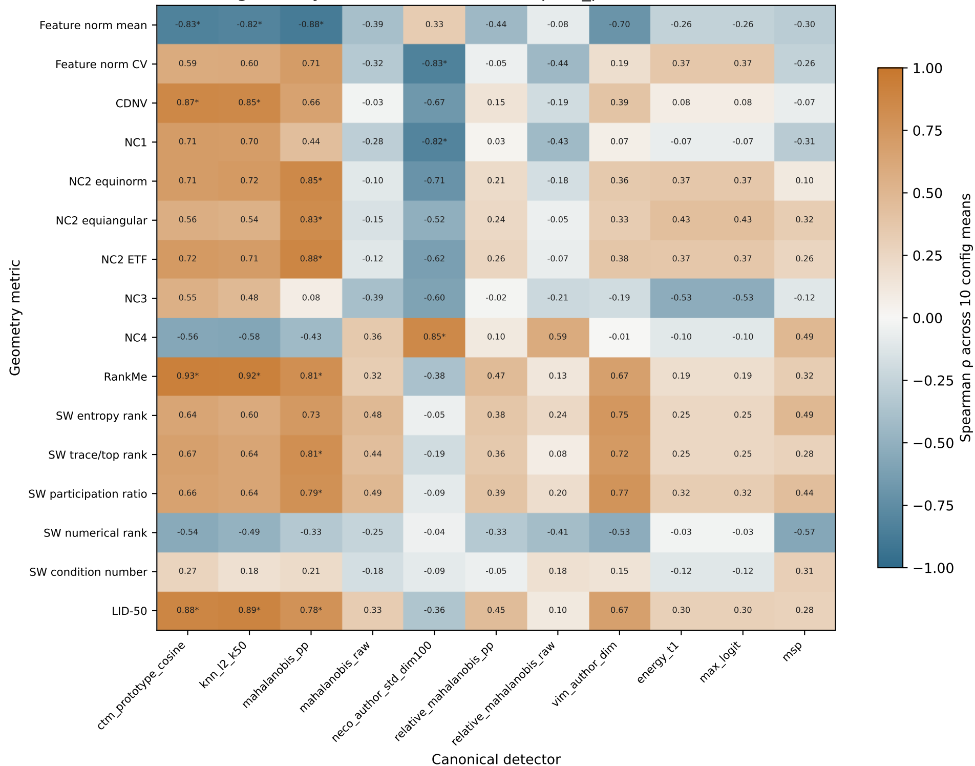
Textures geometry-OOD association (last, fpr95_performance)
