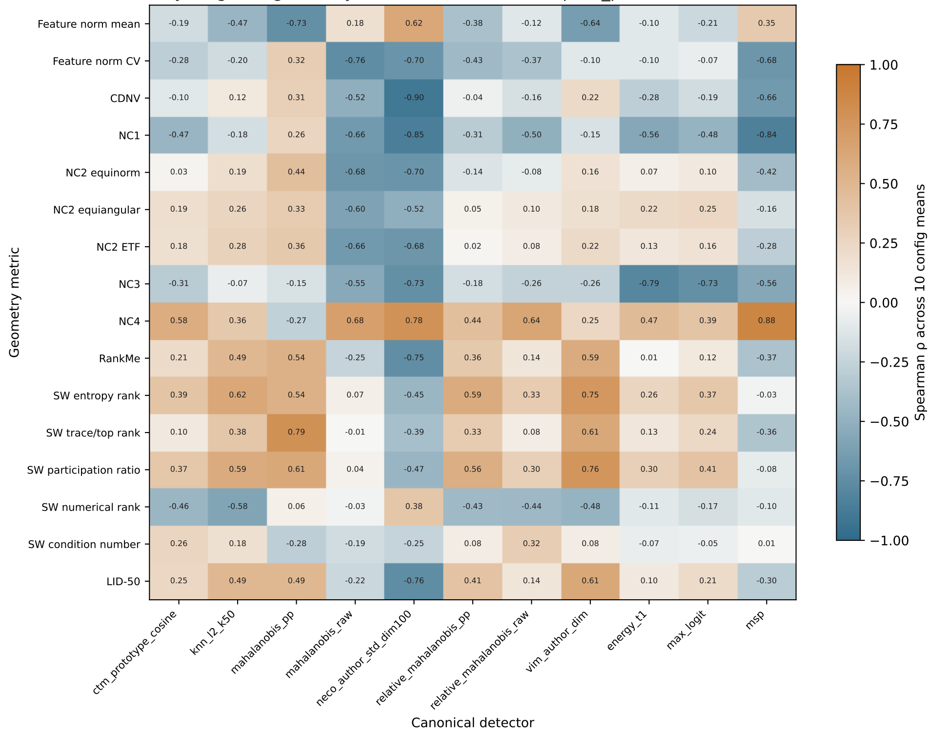
TinyImageNet geometry-OOD association (last, fpr95_performance)
