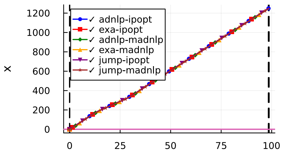
state
