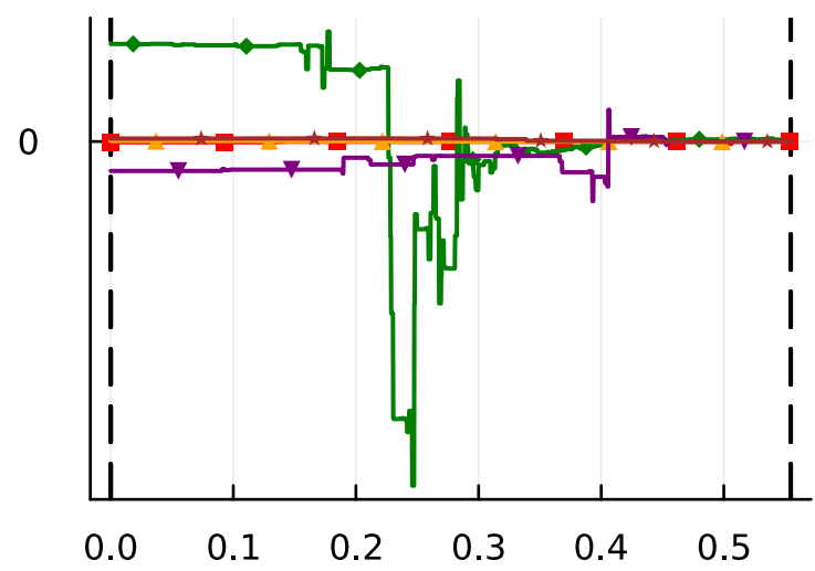
costate
