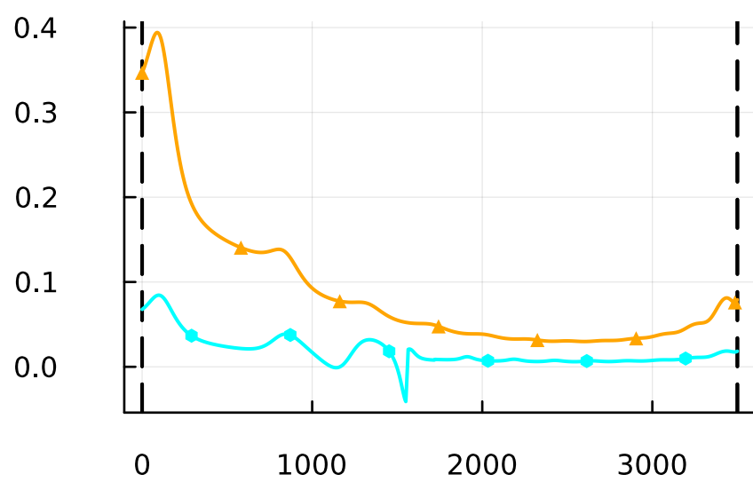
costate
