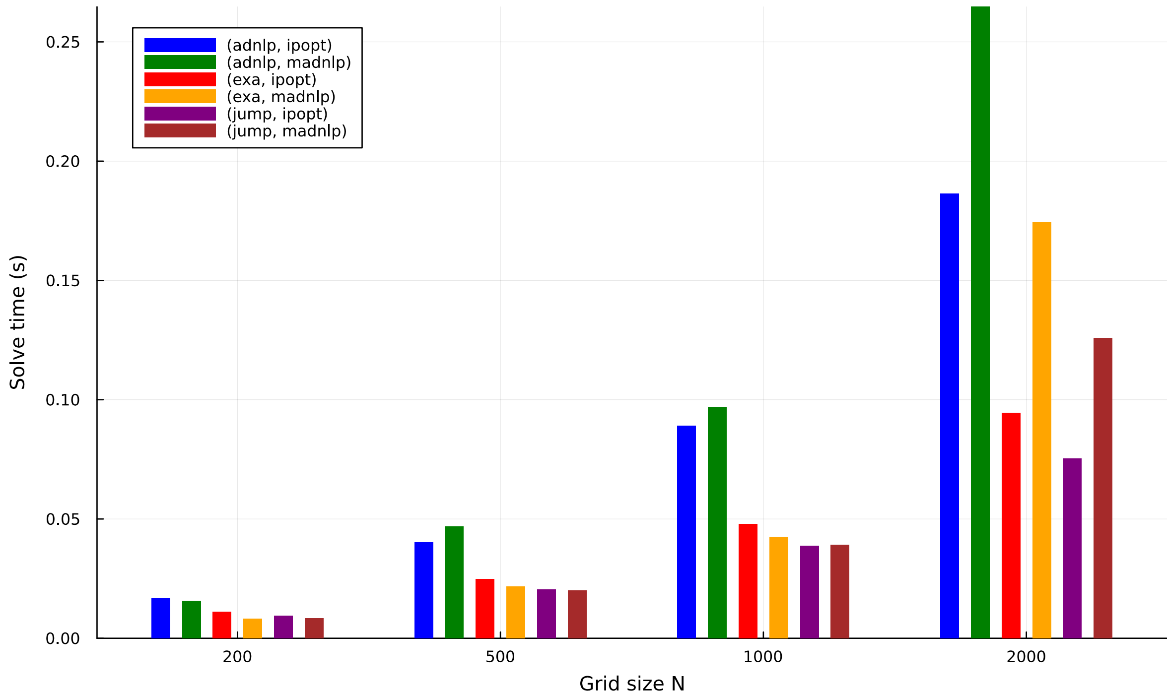
Solve time vs grid size (bar) — double_oscillator
