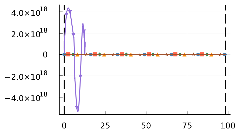
control
