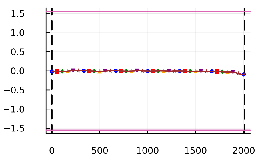
\gamma
