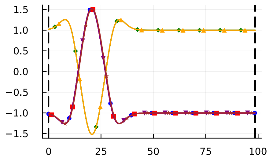
costate
