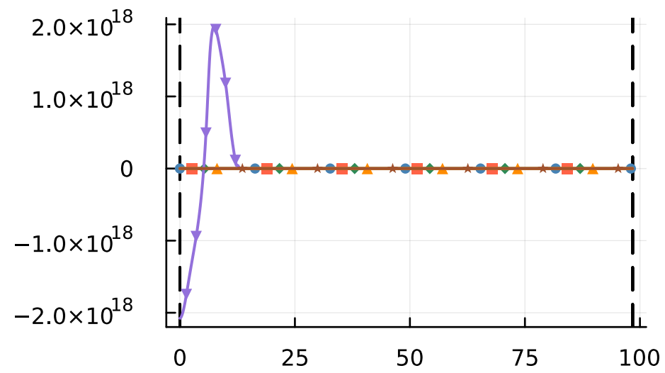
costate
