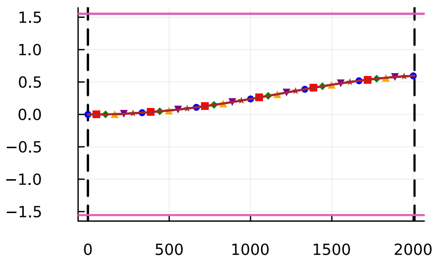
\theta
