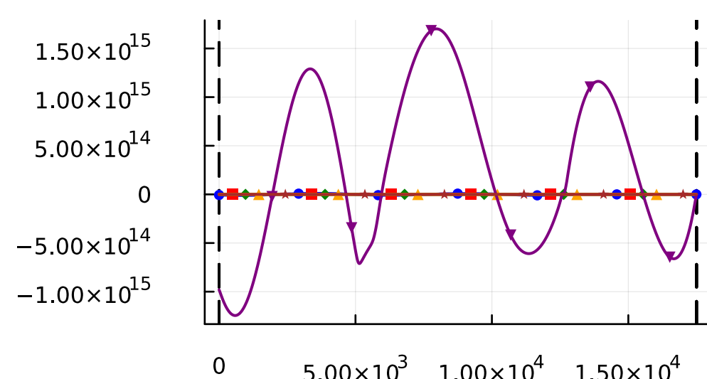
control
