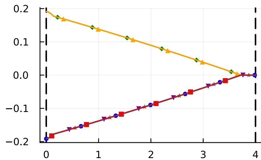
costate
