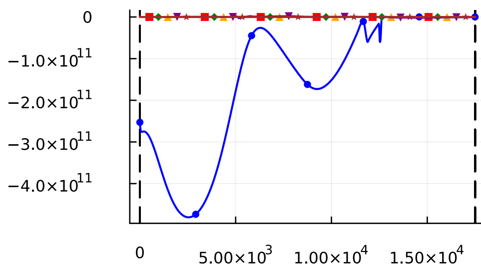
costate
