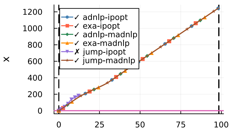
state
