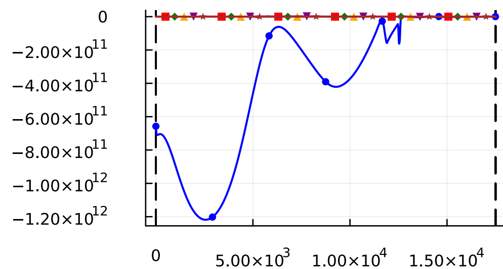
costate
