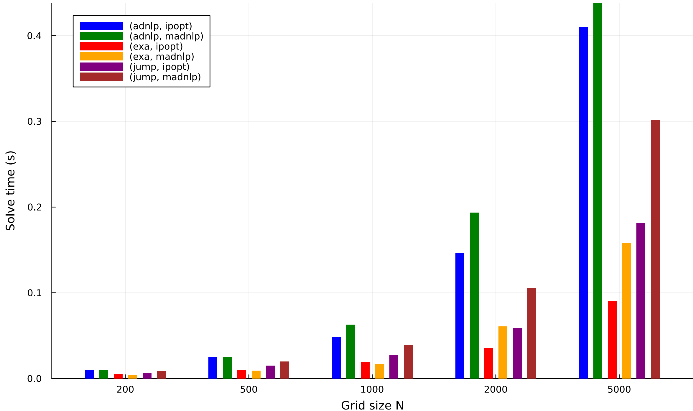
Solve time vs grid size (bar) — electric_vehicle
