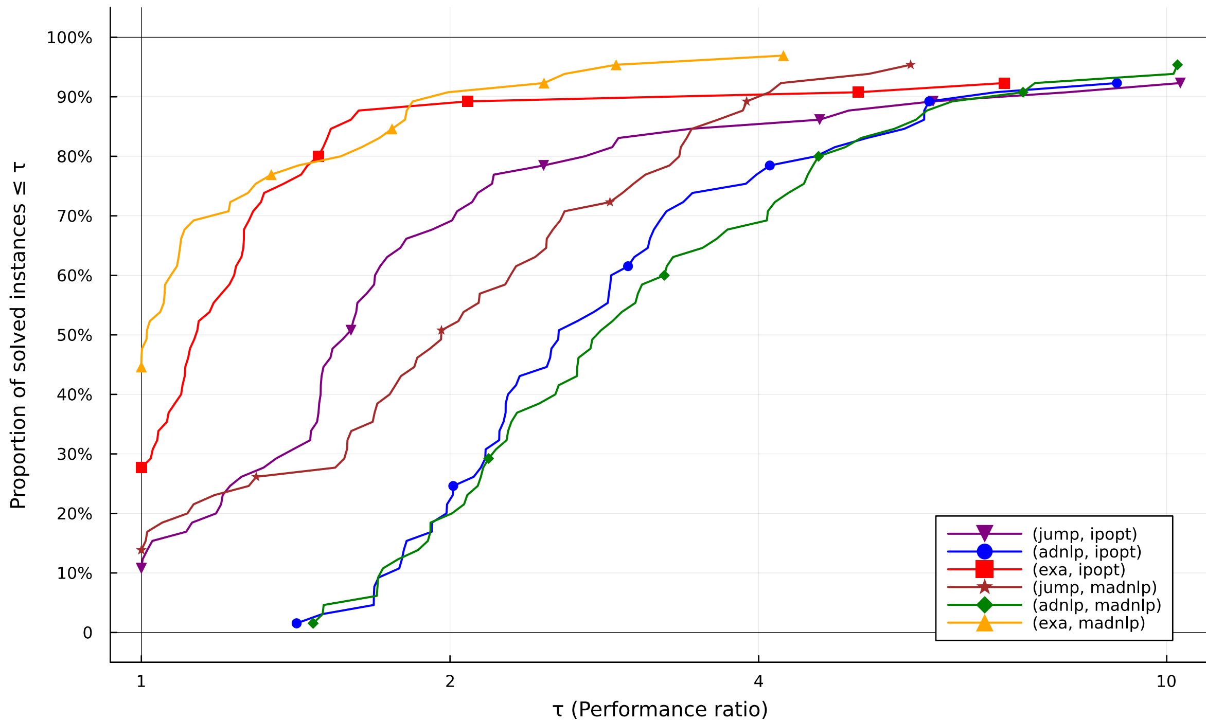
Performance profile — models × solvers
