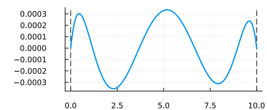
dual
