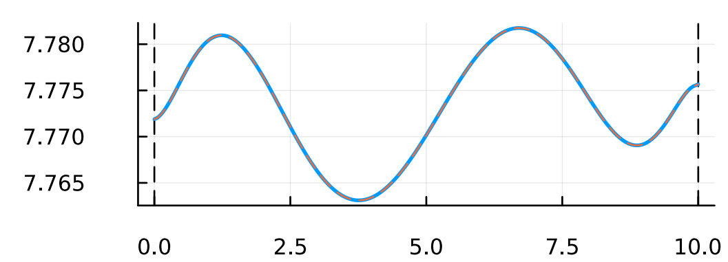
costate
