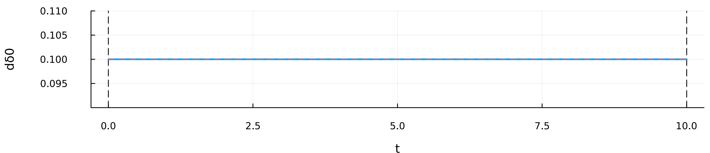
path constraints
