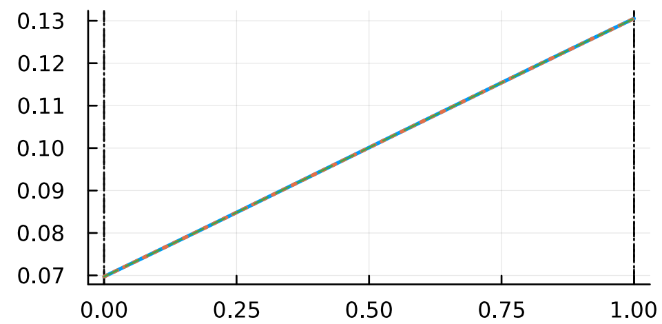
costate
