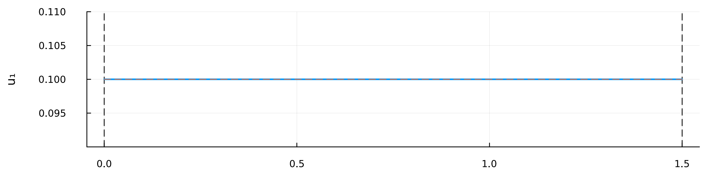
control
