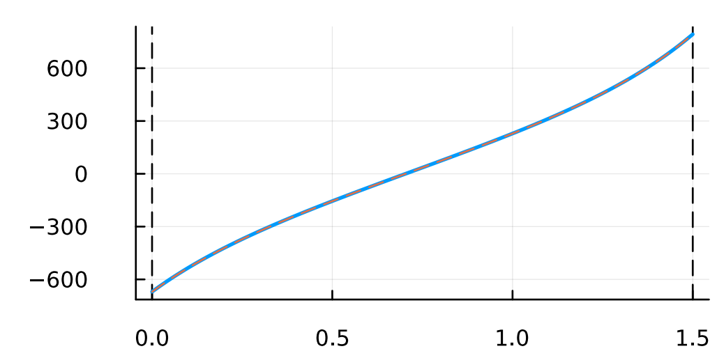
control
