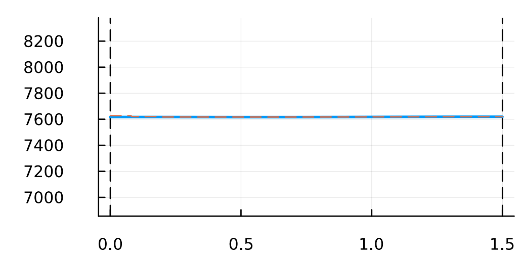
costate
