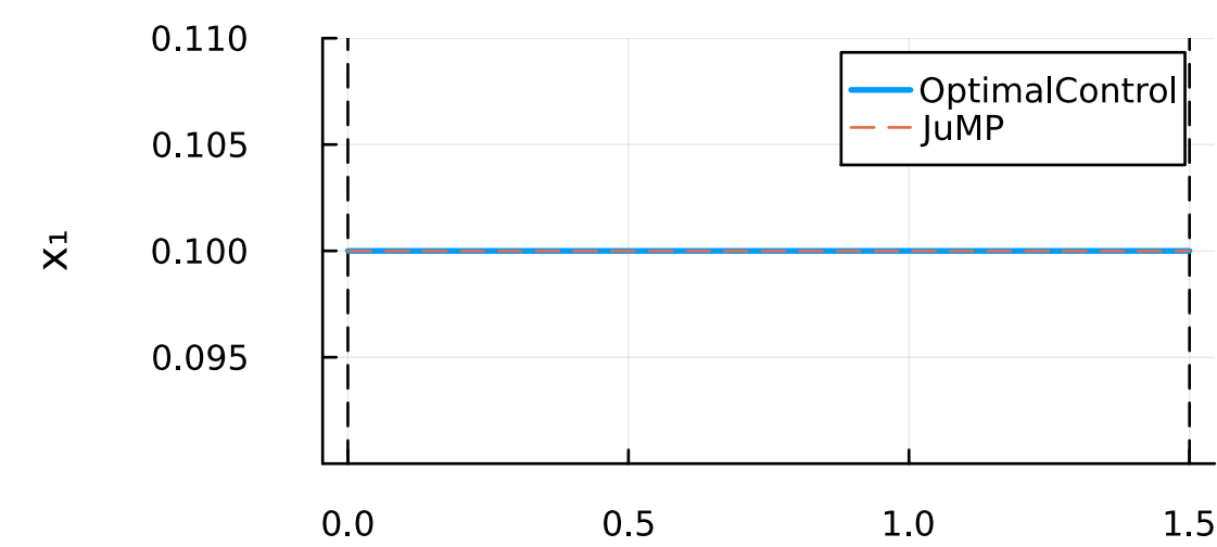
state
