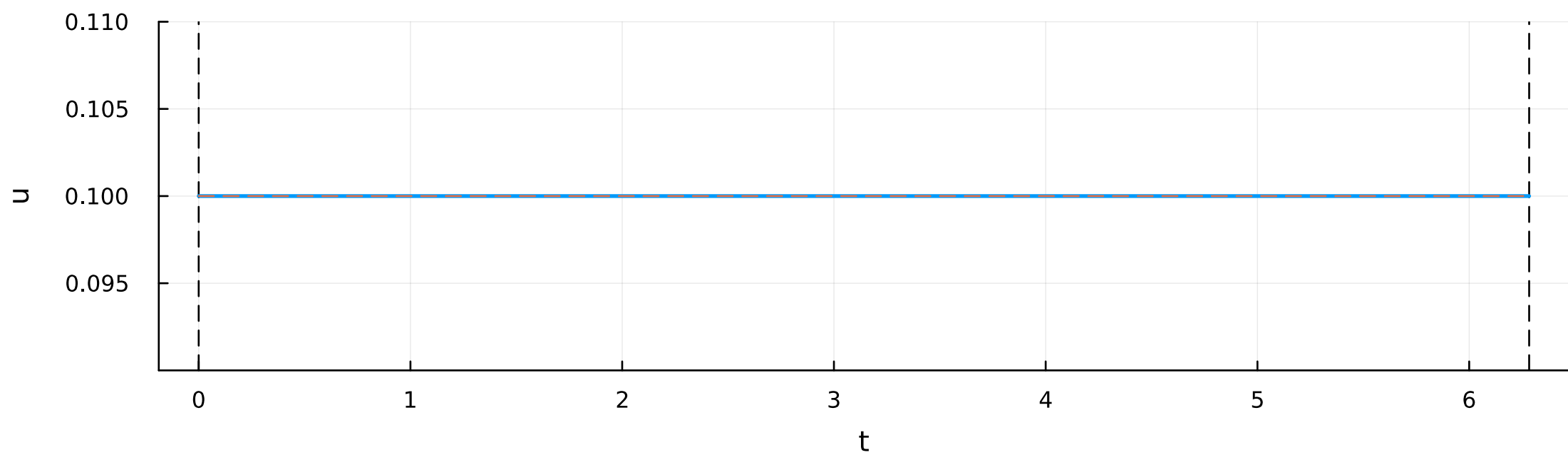
control
