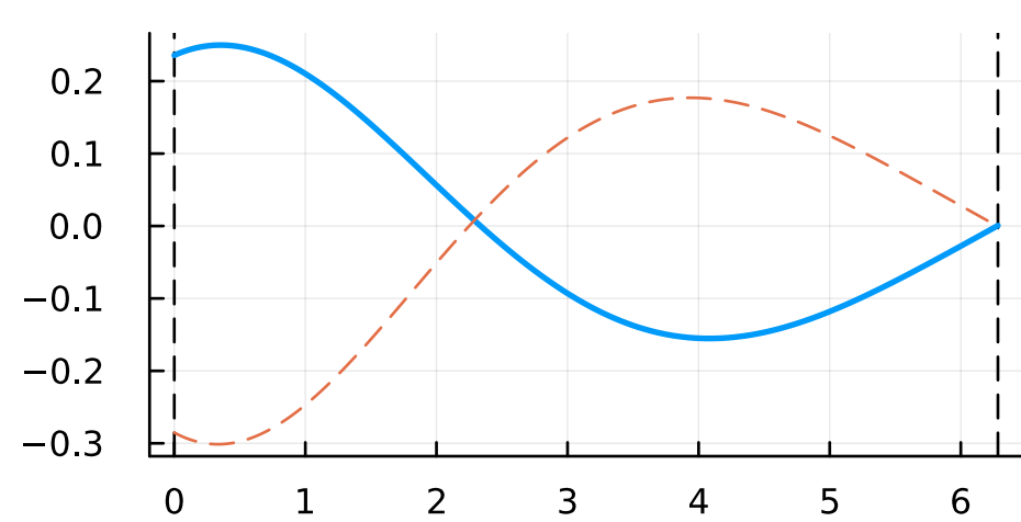
costate
