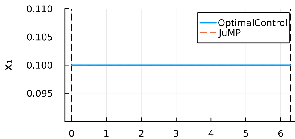
state
