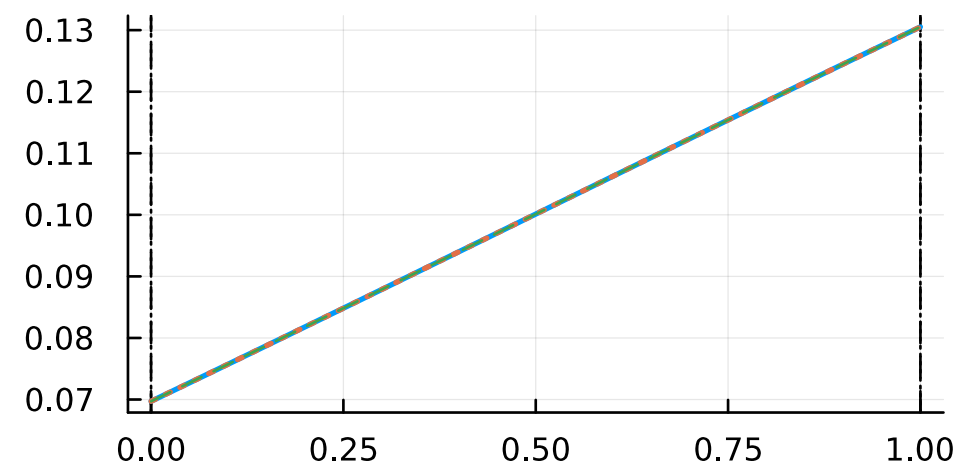
costate
