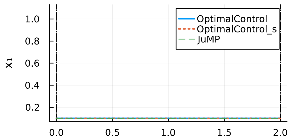
state
