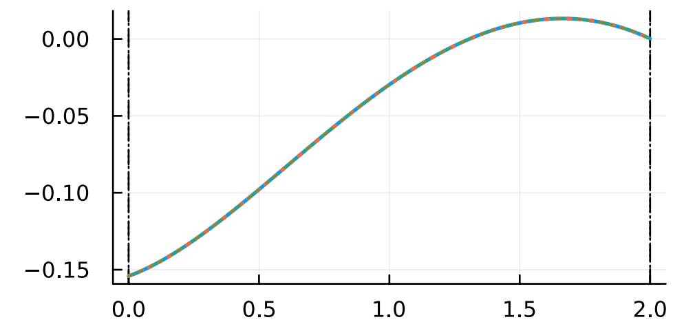
costate
