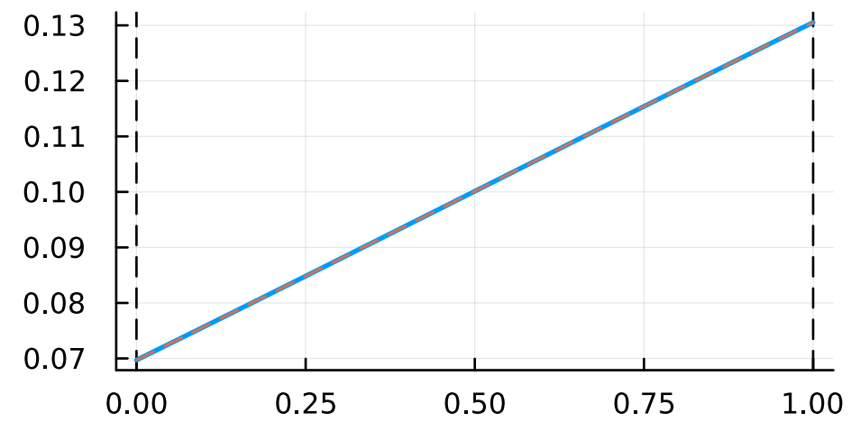
costate
