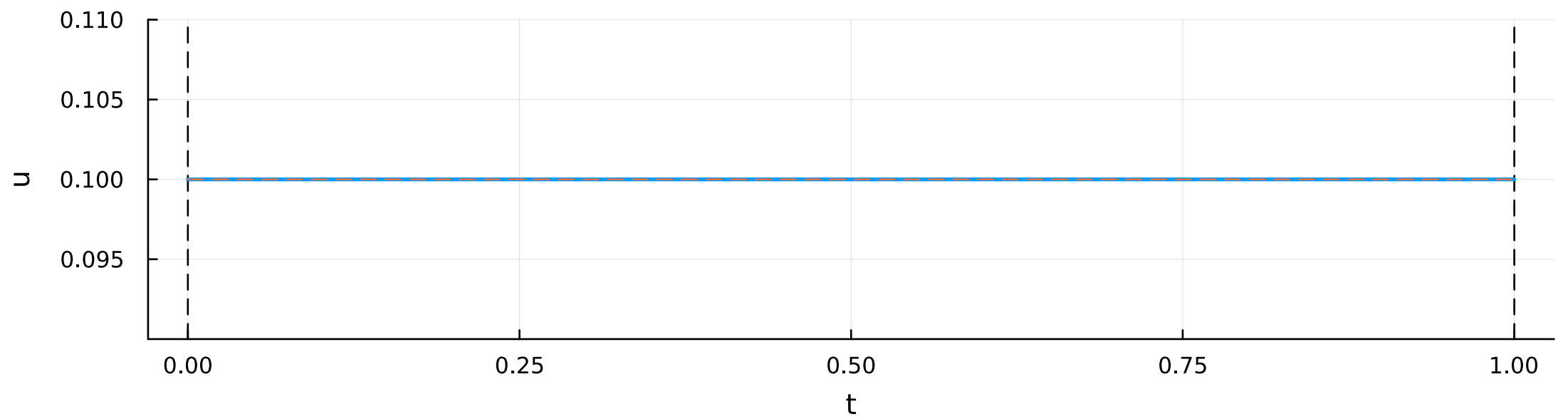
control
