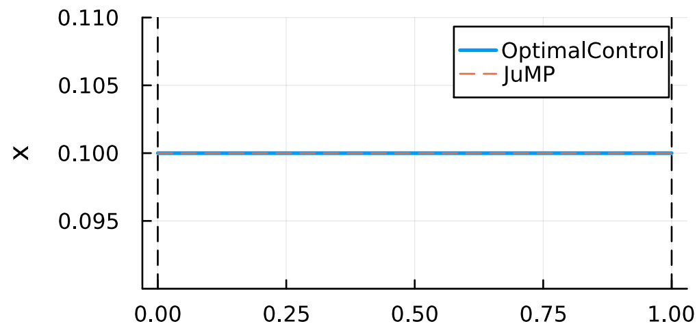
state
