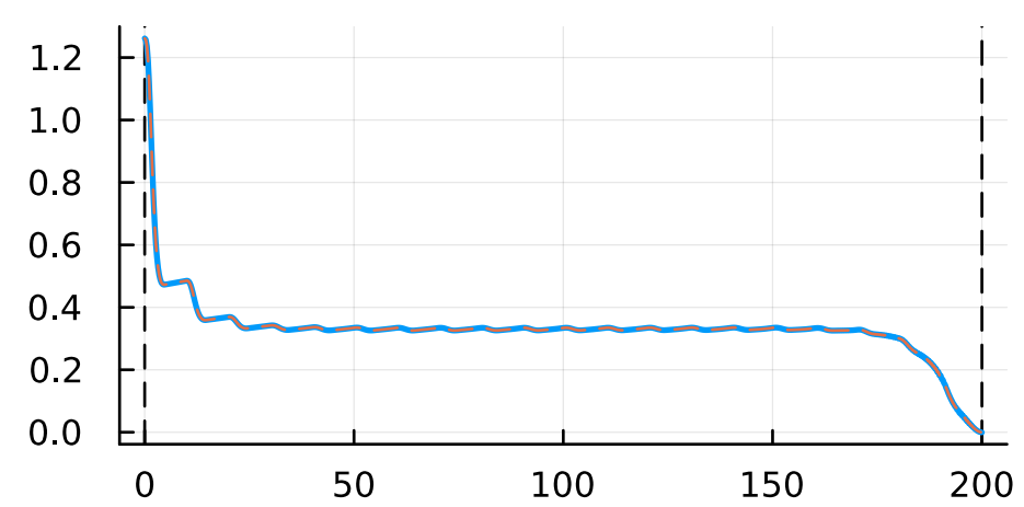
costate
