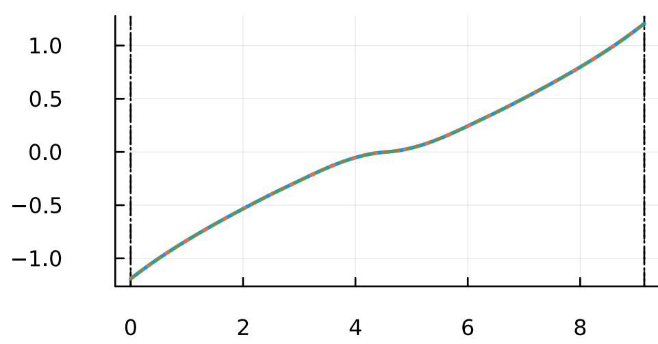
costate
