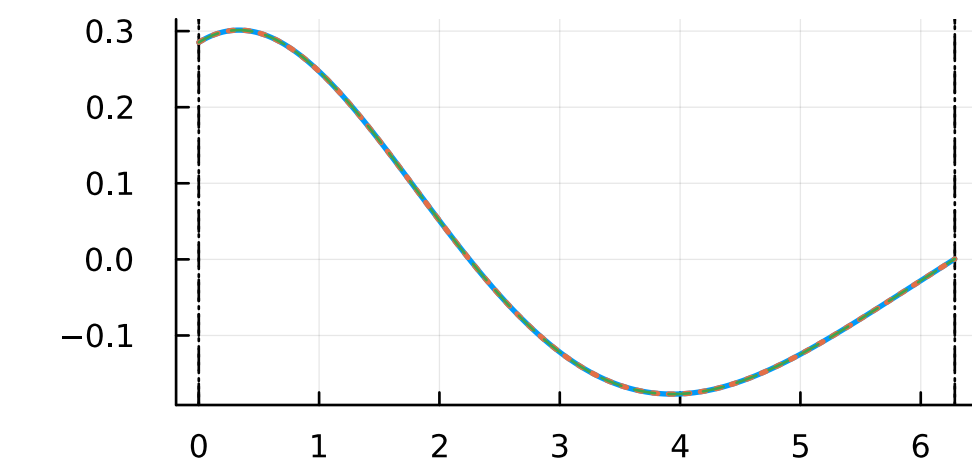
costate
