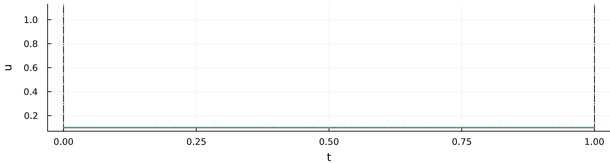
control
