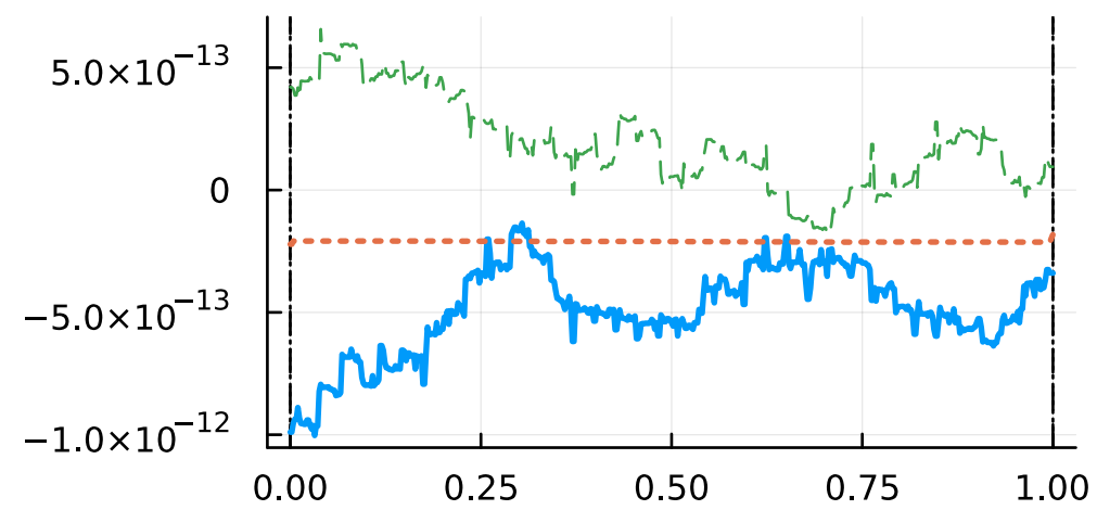
costate
