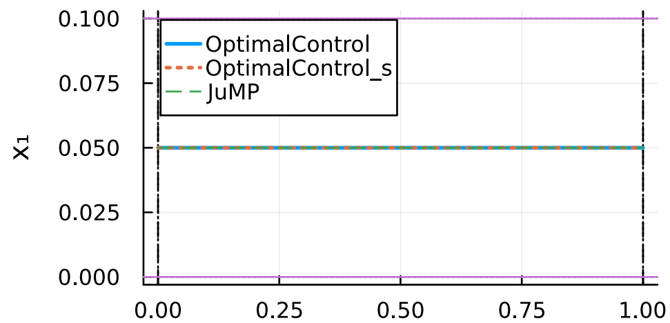
state
