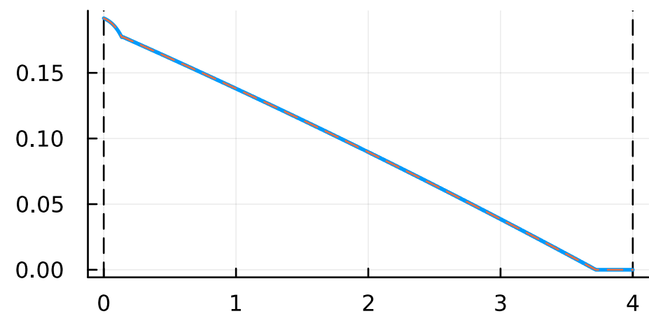
costate
