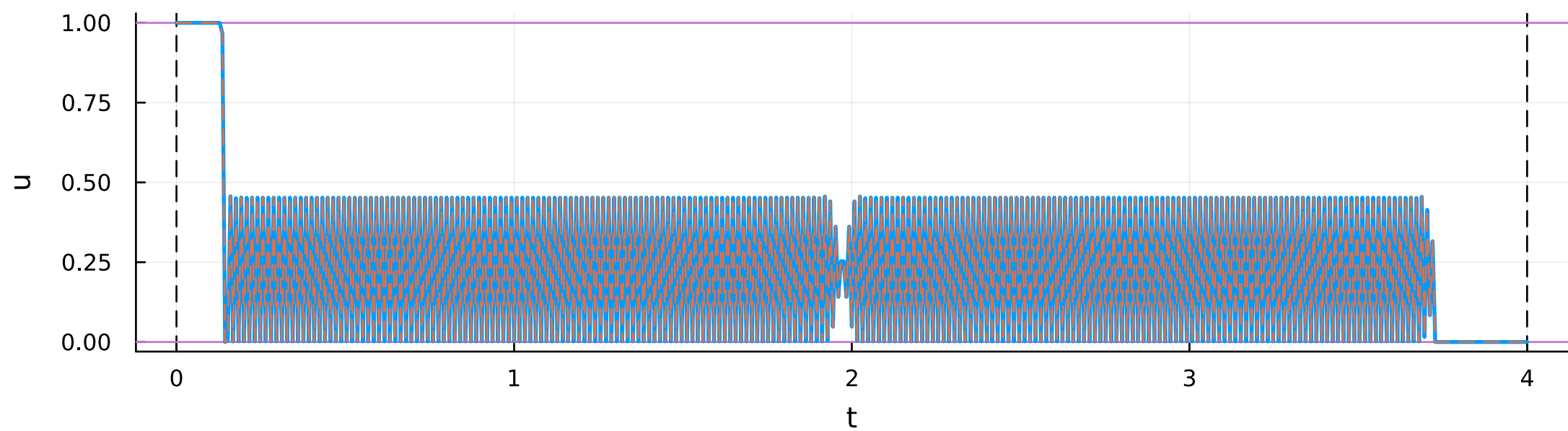
control
