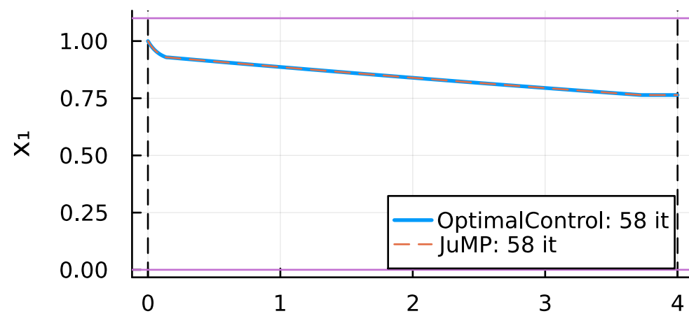
state
