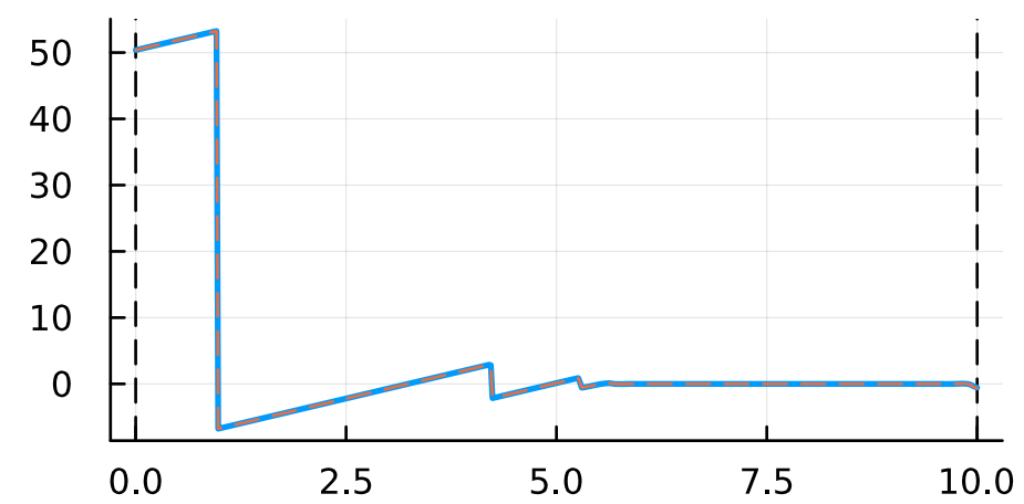
costate
